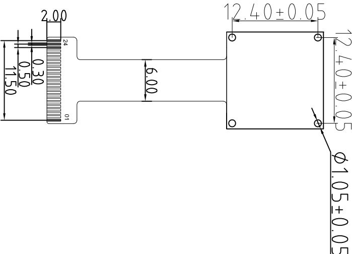
BOTTEM VIEW
